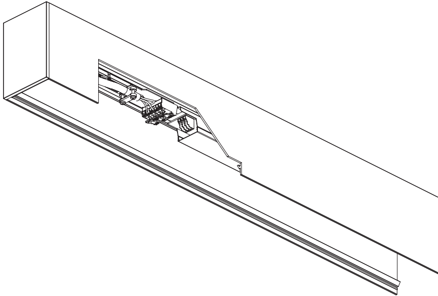
electrical connection
